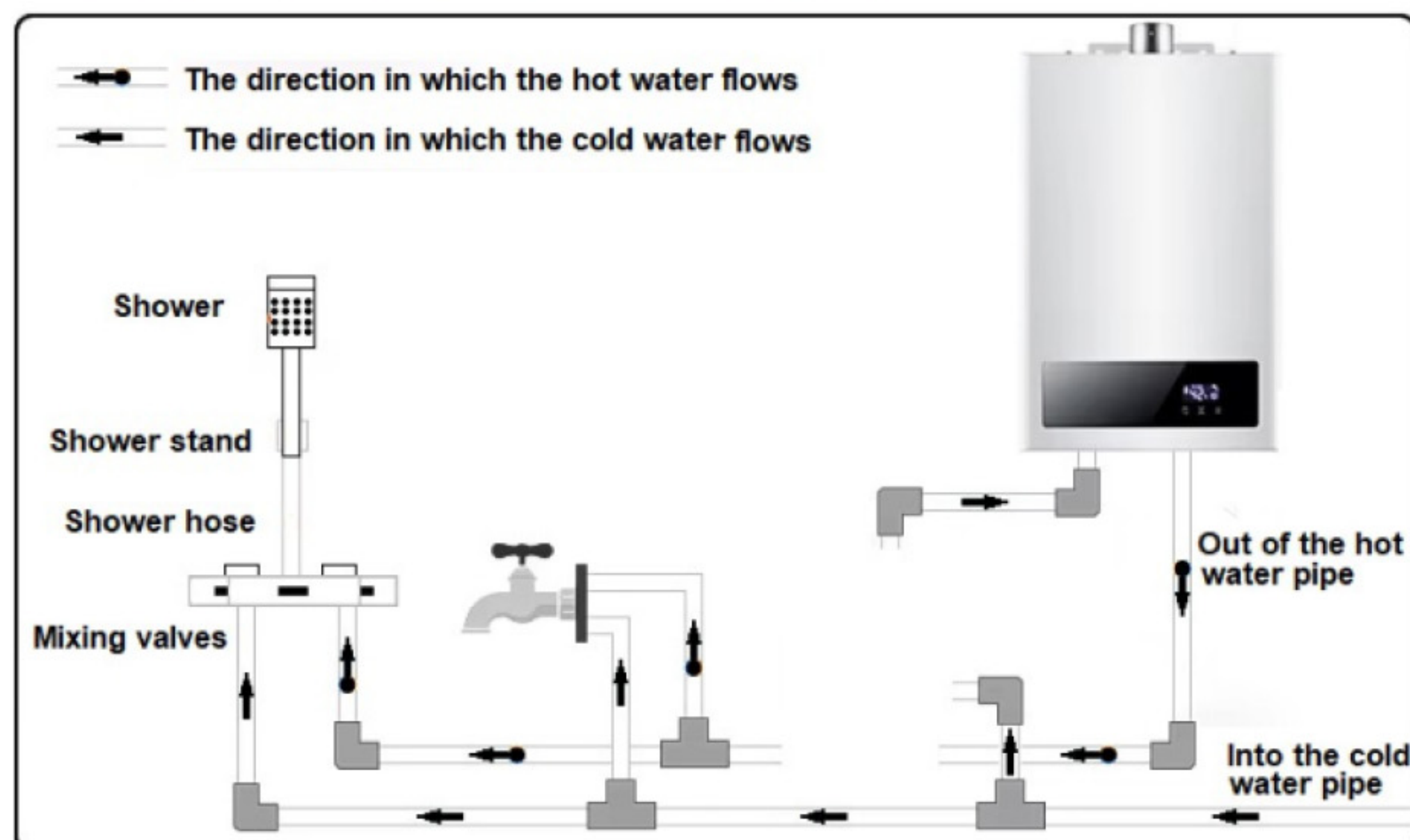
Wall-hung furnace pressurization
